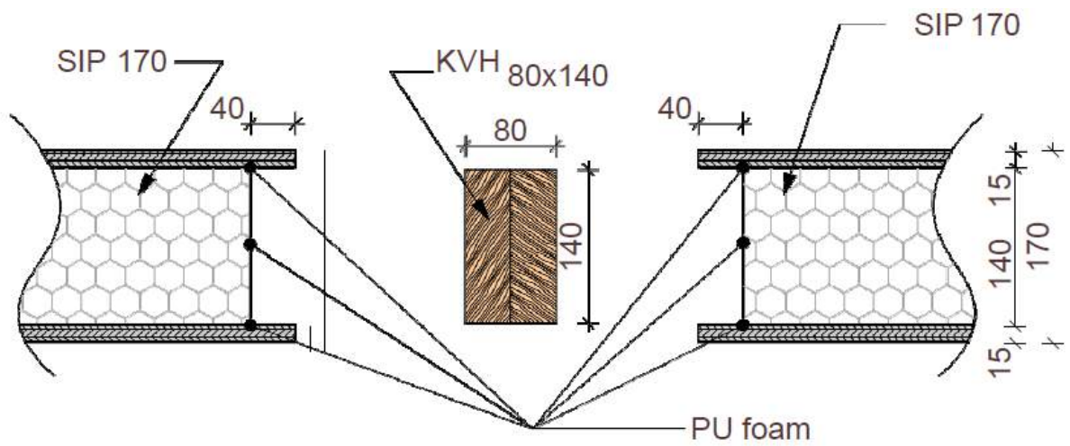
Figure 25 – Joining of the panels by wood components
