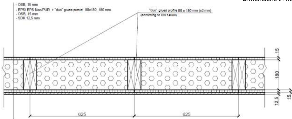
Figure 11 – Floor 1
