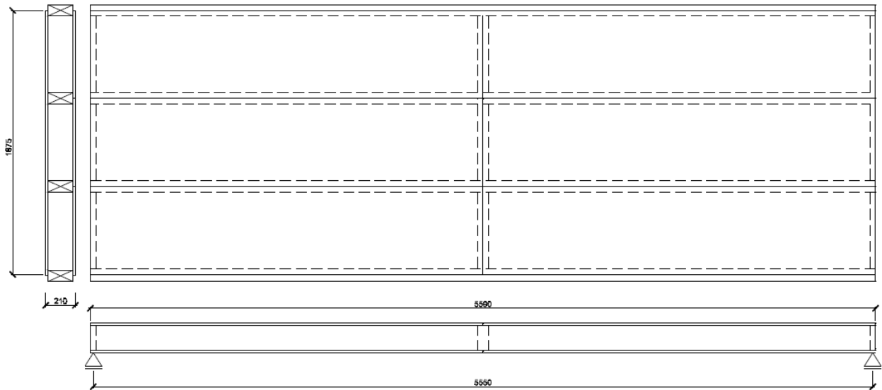
Figure 20 – Racking resistance in floor and roof plain, alternative 1
