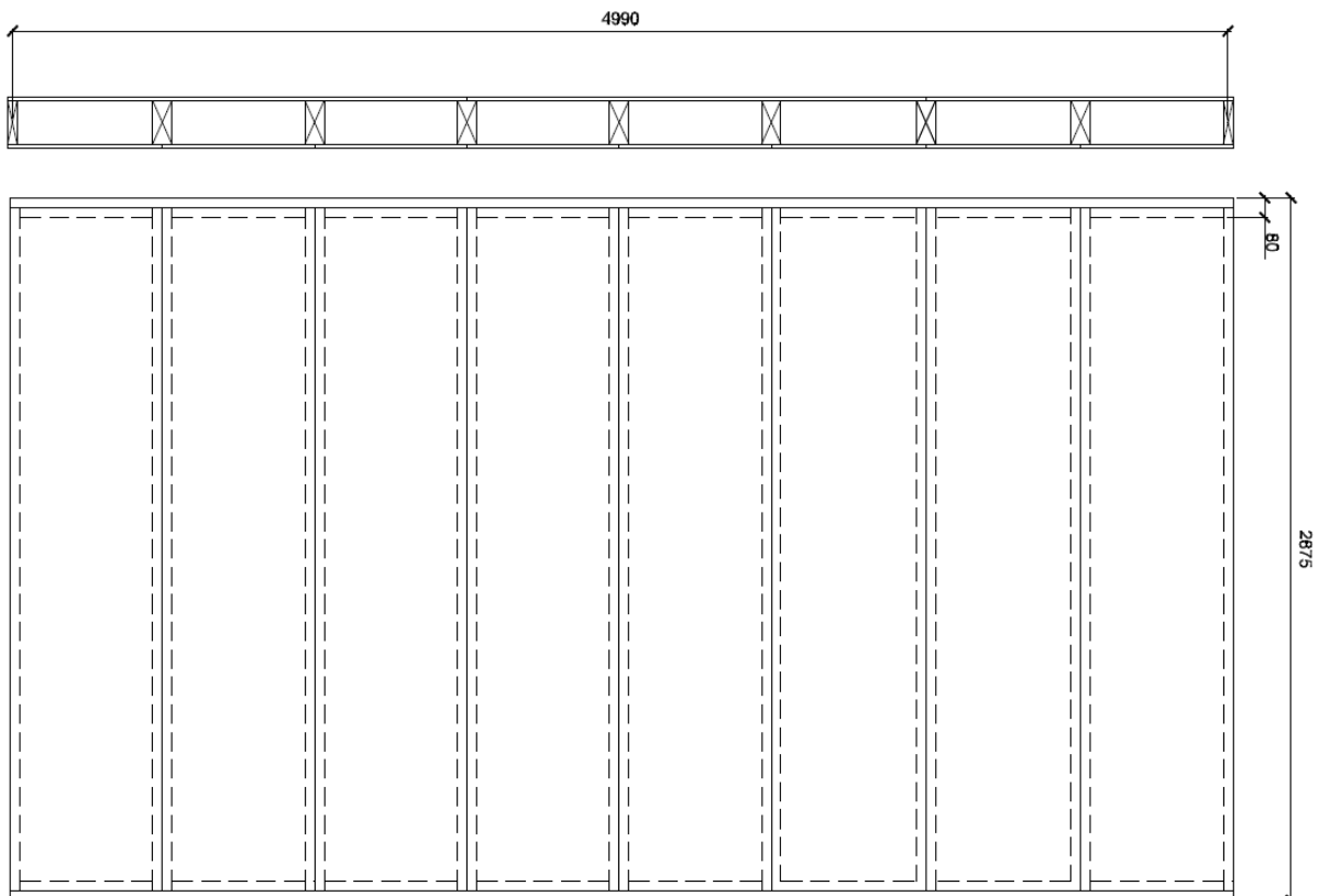
Figure 21 – Racking resistance in floor and roof plain, alternative 2
